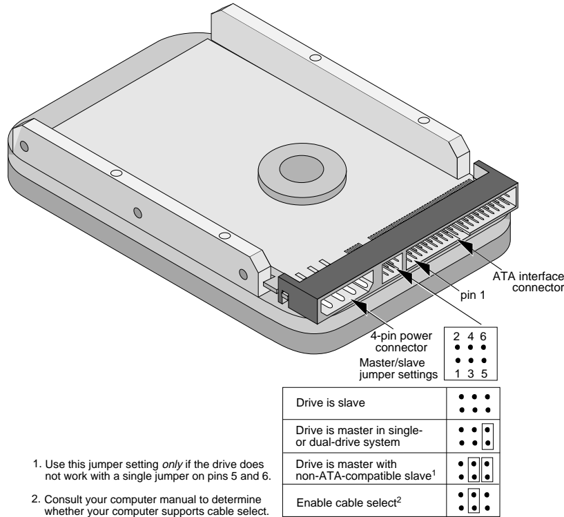
Figure 2. Master/slave jumpers
